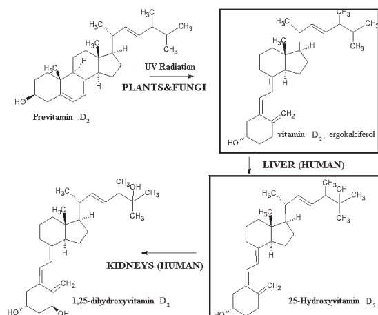
Figure 2. Synthesis of active forms of vitamin D 2 (frames: examples of forms determinable by LC-MS method)
